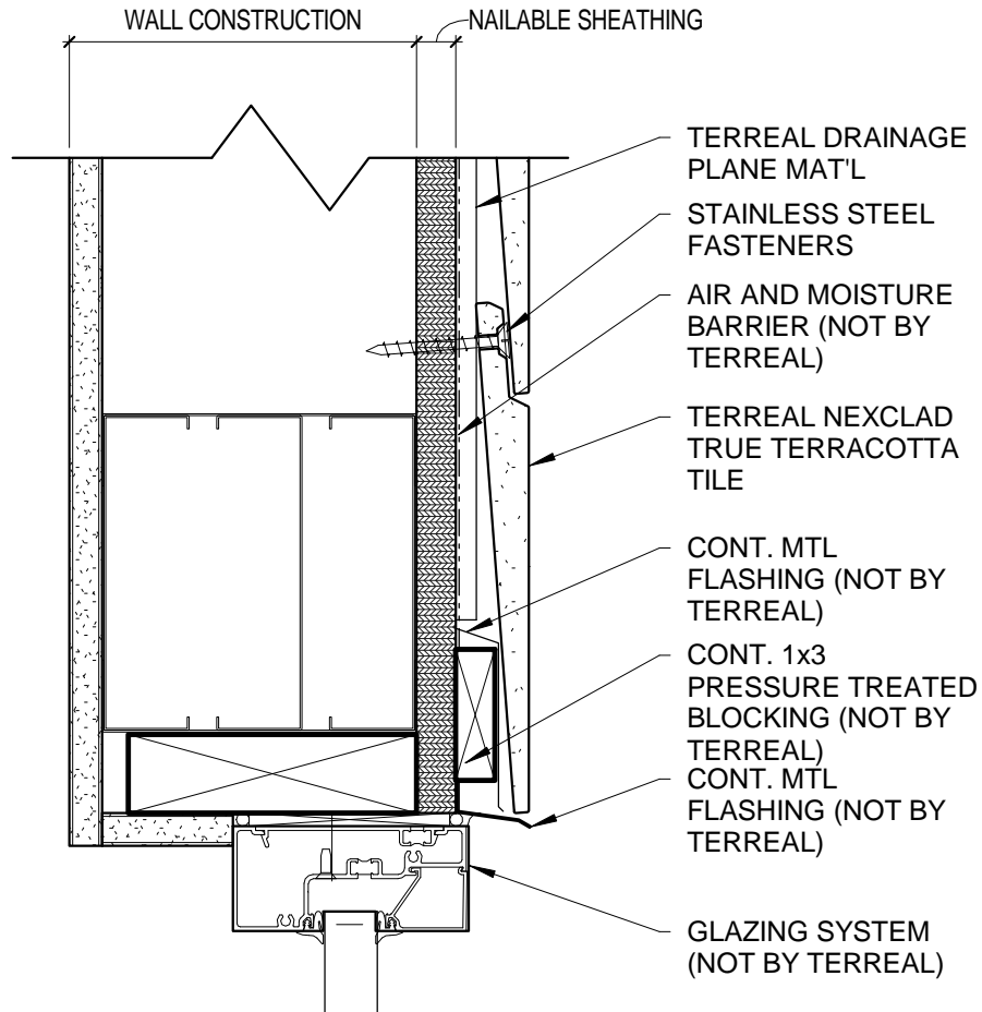
1 SECTION DTL - HEAD 3" = 1'-0"
